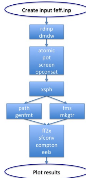
Figure 3.3: Flow chart of the FEFF program showing all submodules. The ldos module is not shown - it can be executed any time after the calculation of the potentials.
